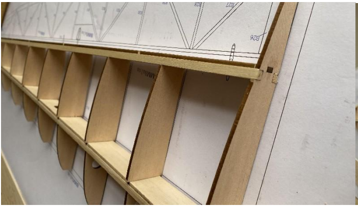
58 Preset the PVC tube(for carbon tube) in the wing.
