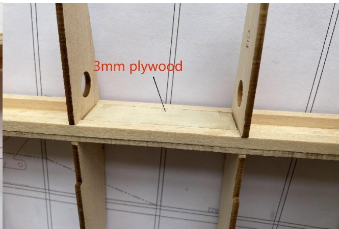
59-60 Two pcs of 3mm plywood are used for reinforcement at the position where the wing strut is attached.
